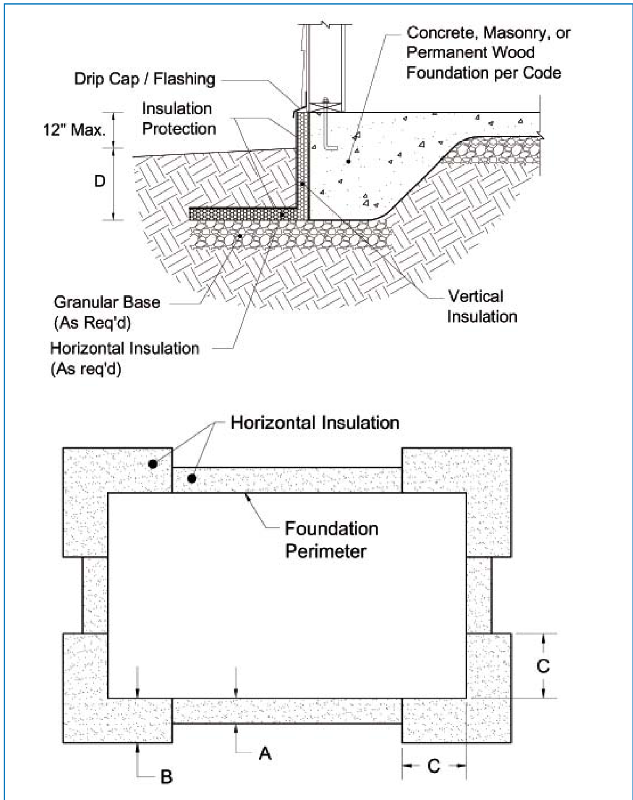
Figure 5. FPSF Simplified Design Parameters – Heated Buildings
