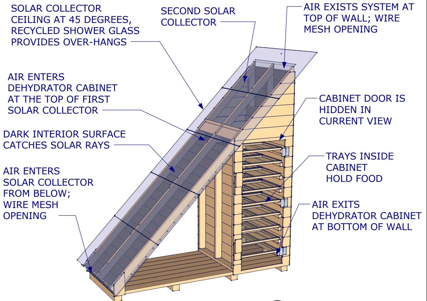
(A8.1) 1 Conceptual Drawing scale: none
